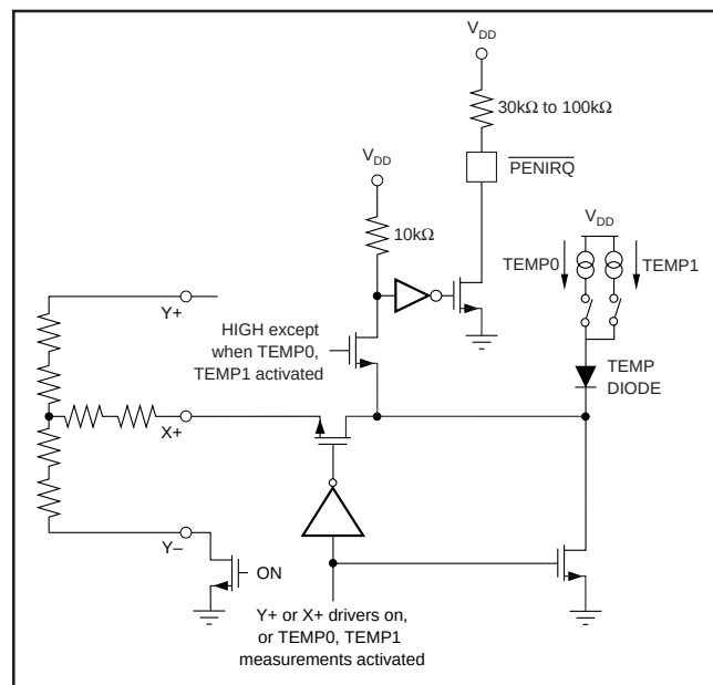
FIGURE 16. PENIRO Functional Block Diagram.
