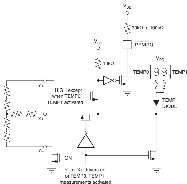
Figure 18. PENIRO Functional Block Diagram
