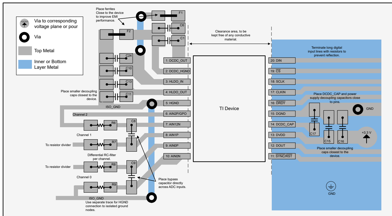
Figure 9-7. Layout Example
