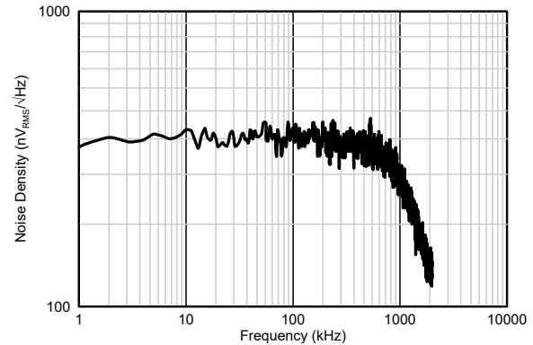
Figure 6-17. Noise Spectral Density vs Frequency
