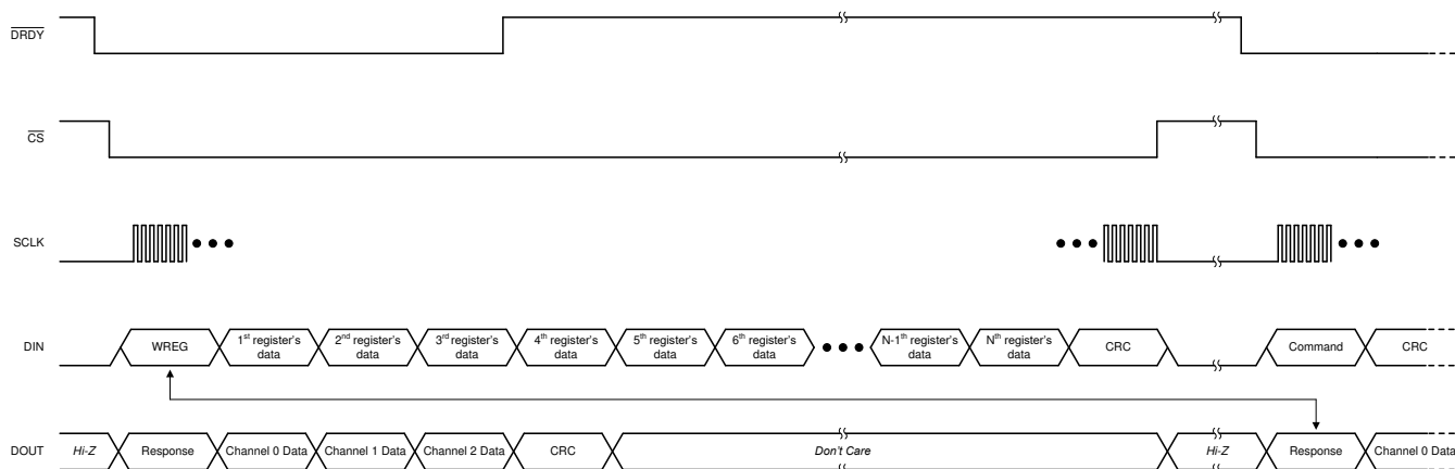
Figure 8-29. Writing Registers
