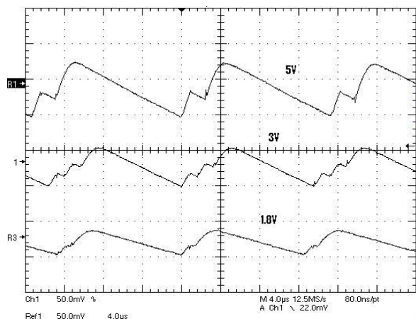
Figure 18. Typical CRD_VCC Ripple Voltage (5 V, 3 V and 1.8 V) – cms Capacitor C_{OUT} = 10 \mu F, 1210, X7R, 16 V
