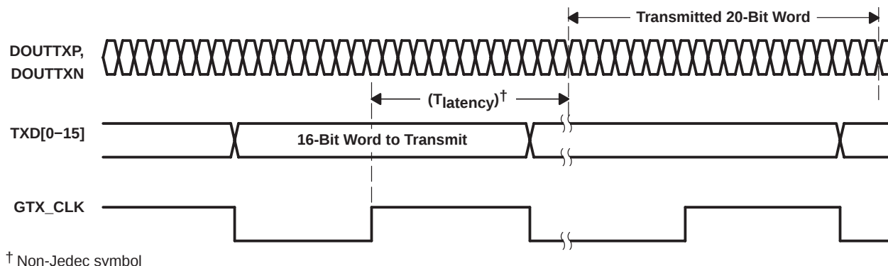
Figure 3. Transmitter Latency
