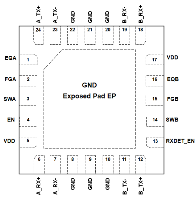
Figure 2. UQFN24 Package Pinout (Top View)
