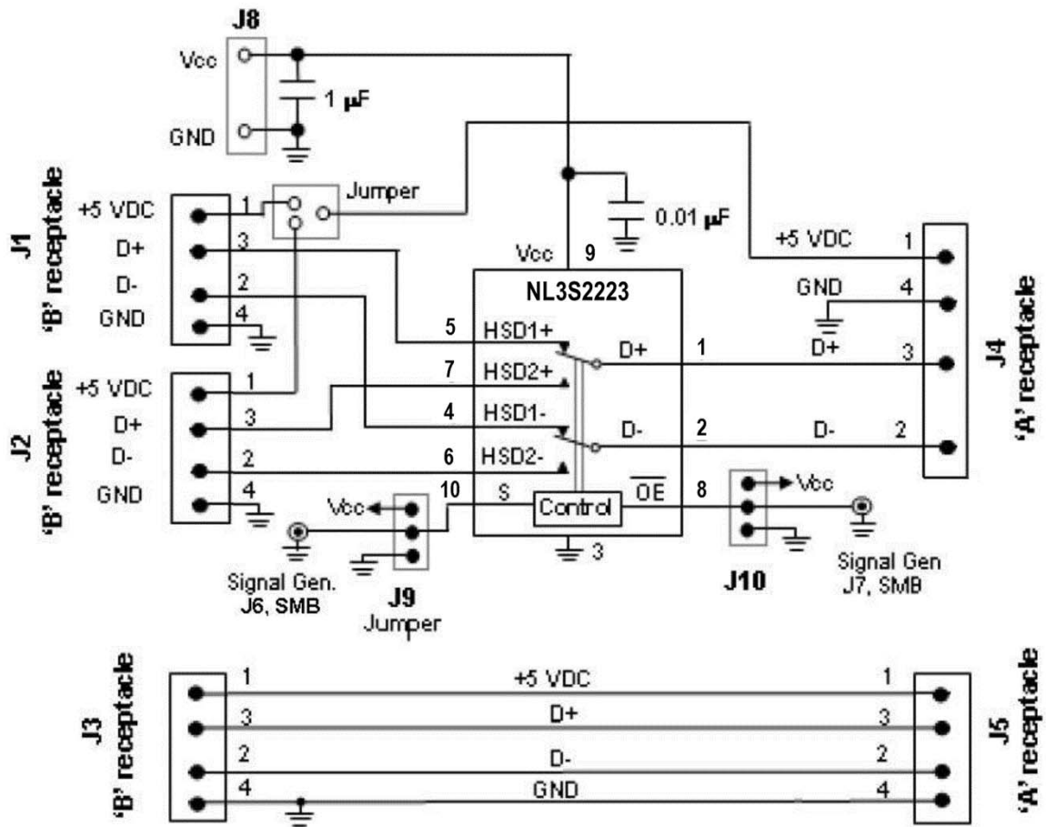
Figure 7. Board Schematic
