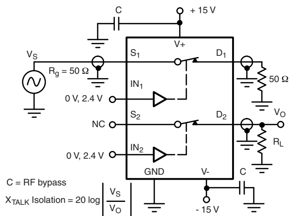
Figure 4. Channel-to-Channel Crosstalk
