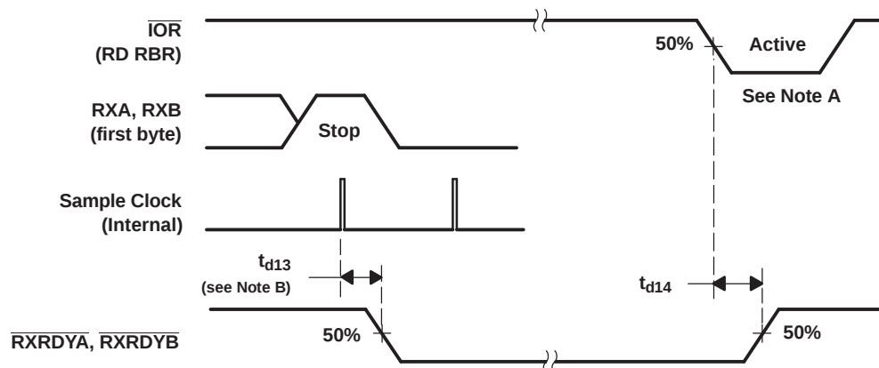
Figure 11. Receiver Ready (RXRDY) Waveforms, FCR0 = 0 or FCR0 = 1 and FCR3 = 0 (Mode 0)
