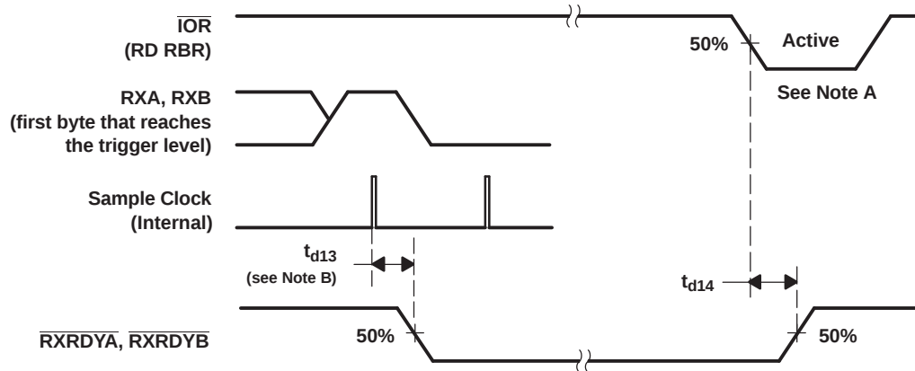
Figure 12. Receiver Ready (RXRDY) Waveforms, FCR0 = 1 and FCR3 = 1 (Mode 1)
