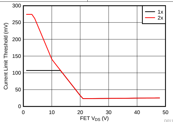
Figure 11. Foldback Current Limit Threshold ( V_{LIM} , V_{LIM2X} ) vs Port MOSFET Voltage
