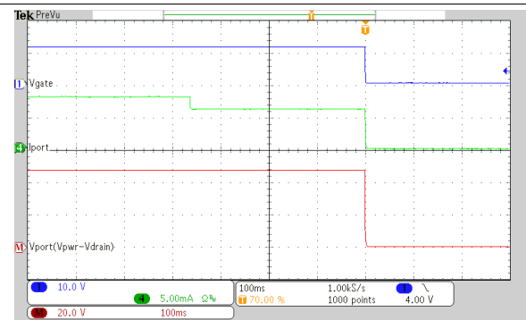
Figure 91. Response to 8-mA to 6-mA Load, DC Disconnect Enabled
