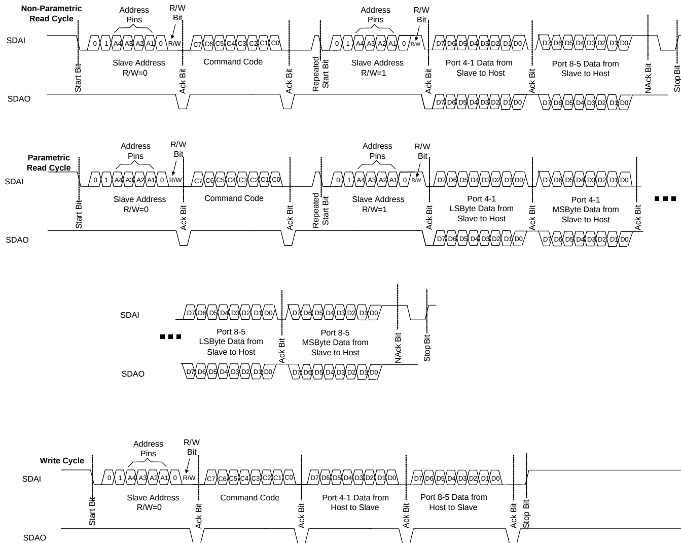
Figure 20. I²C interface Read and Write Protocol – Configuration B
