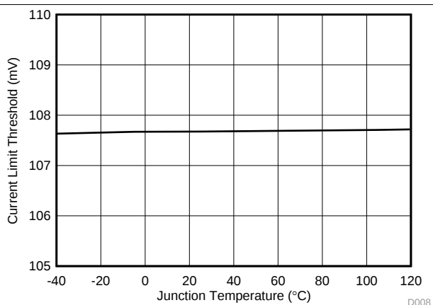
Figure 8. Current Limit 1x Threshold ( V_{LIM} ) vs Junction Temperature
