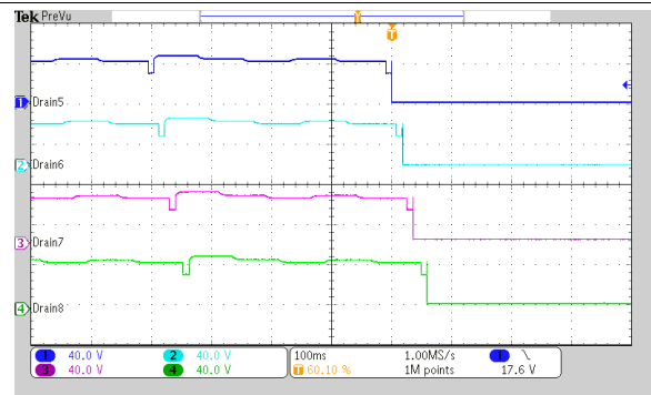
Figure 79. All Ports Power-On With TPON Bit Set
