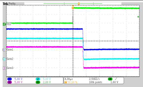
Figure 78. Powering Up into a 100-μF Load
