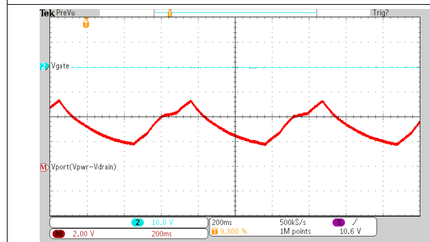
Figure 74. Detection With Invalid PD (15 k \Omega and 0.1 \mu F)
