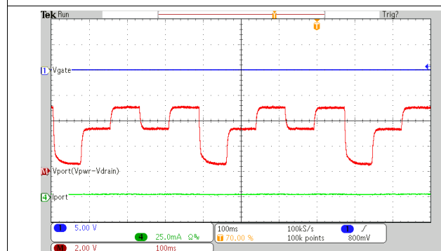
Figure 72. Startup With Valid PD (25 k \Omega and 0.1 \mu F), Class 0
