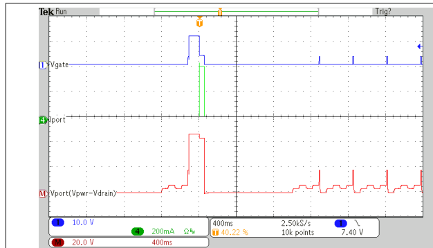
Figure 90. Current Limit Timeout Restart Delay
