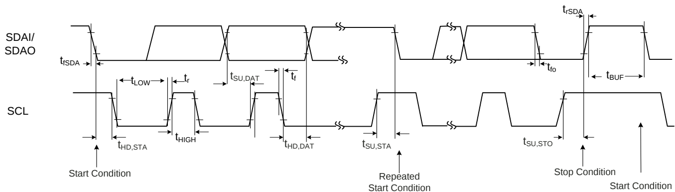
Figure 12. I²C Timings
