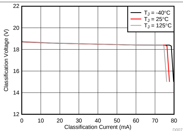
Figure 7. Classification Voltage ( V_{CLASS} ) vs Port Classification Current
