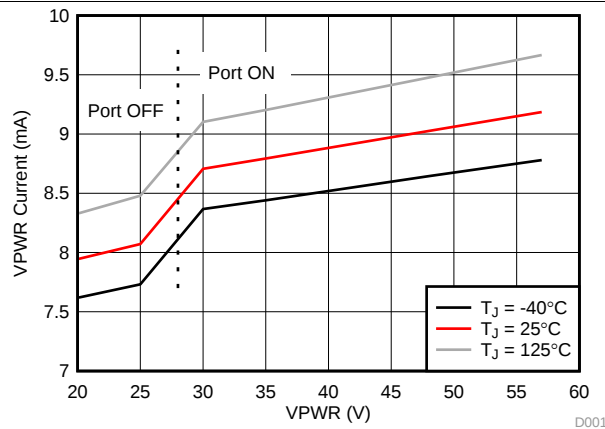
Figure 1. VPWR Current Consumption vs VPWR
