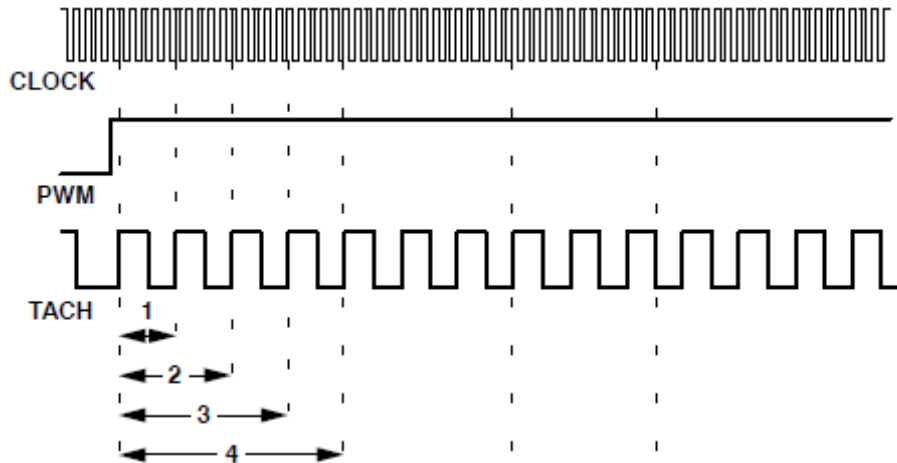
Figure 21. Fan Speed Measurement
