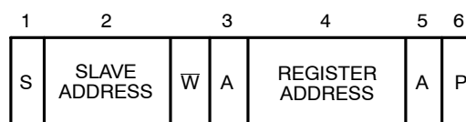
Figure 7. Setting a Register Address for Subsequent Read
