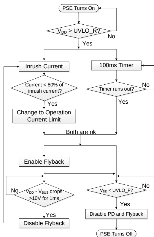
Figure 2: Start-Up Sequence
