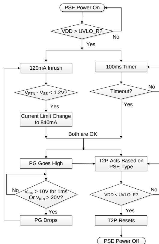
Figure 3: Start-Up Sequence
