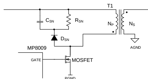
Figure 14: RCD Snubber
