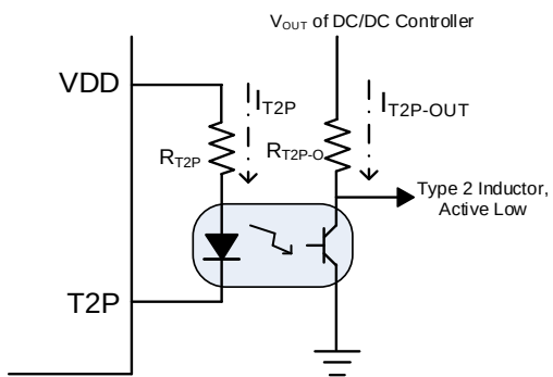
Figure 10: T2P Indicator Circuit
