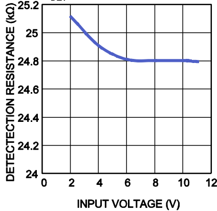
Detection Resistance vs. Input Voltage R DET =24.9kΩ
