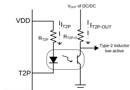
Figure 6: T2P Inductor Circuit
