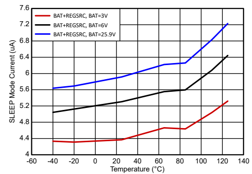
No communications, REGOUT disabled Figure 6-27. Supply Current in SLEEP Mode vs. Temperature
