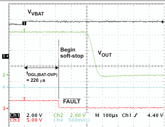
Figure 22. BAT-OVP, V_{BAT} Steps from 4.2 V to 4.4 V, Shows t_{DGL(BAT-OVP)} and Soft-Stop
