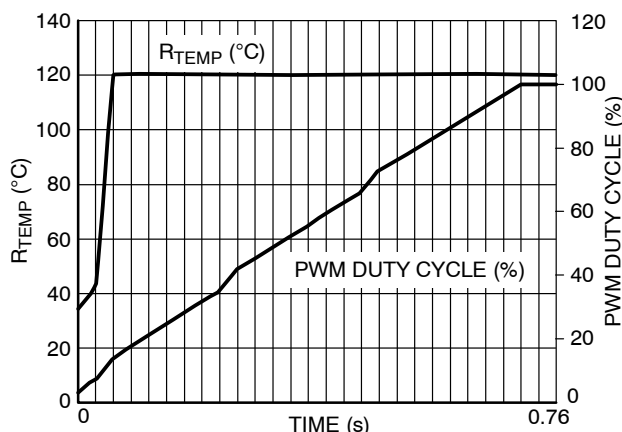
Figure 75. Enhanced Acoustics Mode with Ramp Rate = 48
