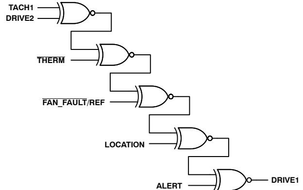
Figure 43. XOR Tree Test
