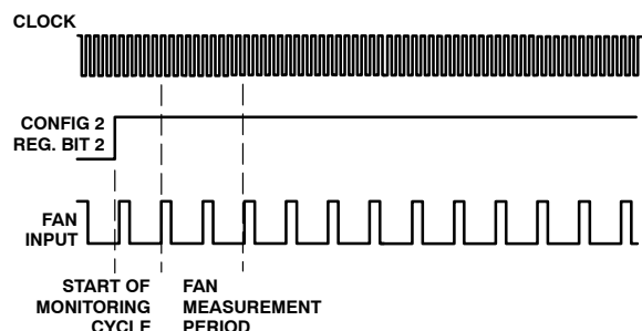
Figure 37. Fan Speed Measurement
