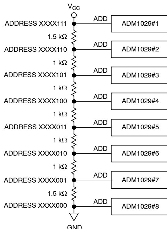
Figure 17. Setting Address of up to Eight ADM1029s
