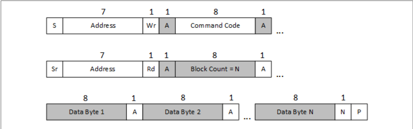
Figure 25 Block Read
