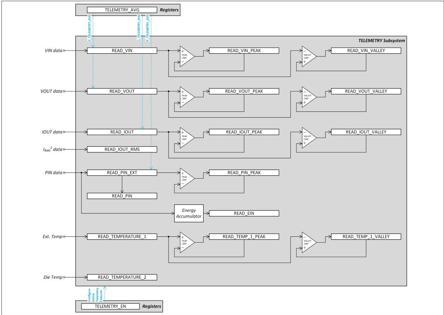
Figure 11 Telemetry flow
