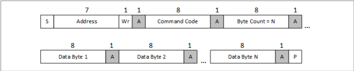
Figure 23 Block Write
