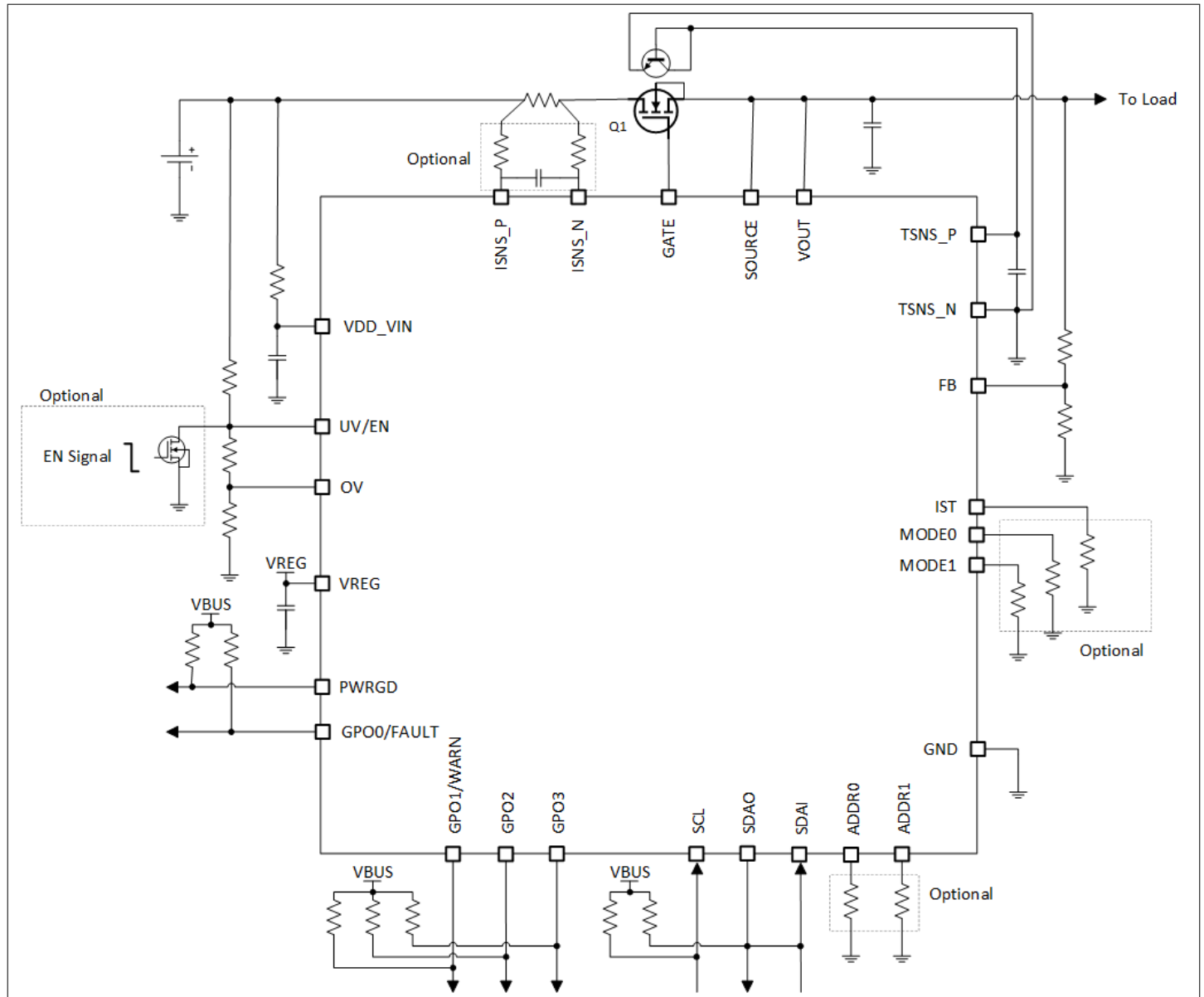
Figure 33 Analog assisted digital mode application schematic
