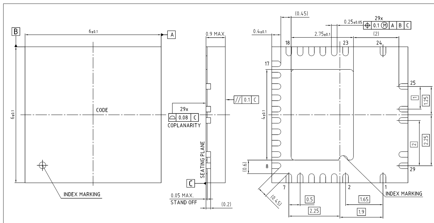
Figure 3 Package dimensions
