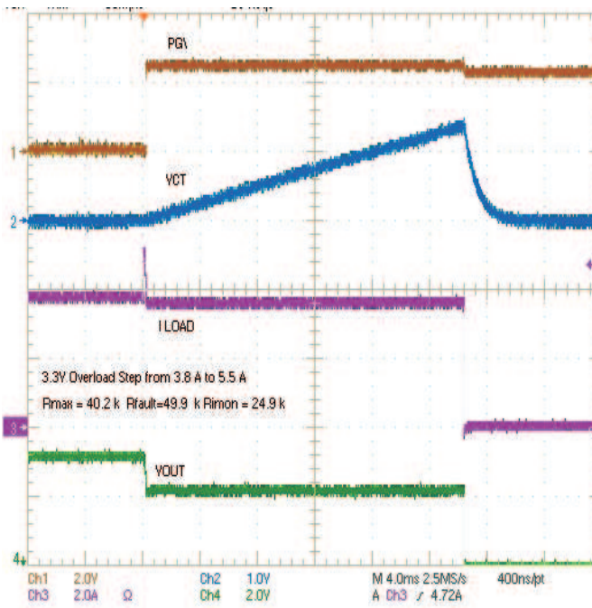
Figure 16. Firm Overload, Load Stepped From 3.8 A to 5.5 A
