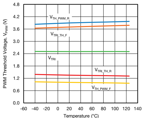
Fig. 7 - PWM Threshold vs. Temperature
