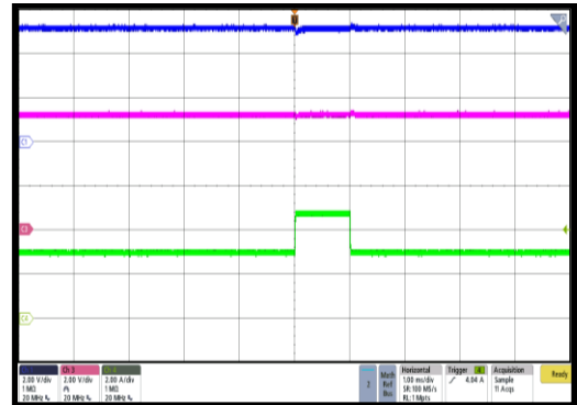
USB2 Load Transient
