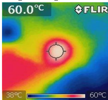
Thermal Imaging V_{IN} = 12V , V_{OUT} = 5.17V , T_A = 25^\circ C , USB1 I_{OUT} = USB2 I_{OUT} = 2.4A
