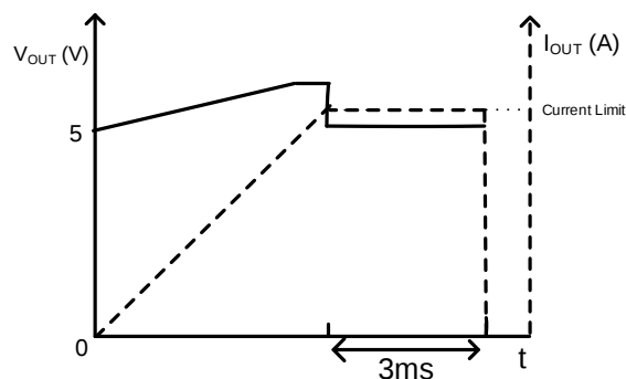
Figure 7: Over-Current Limit
