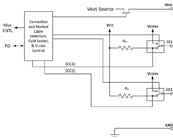
Figure 9: CC Functional Block
