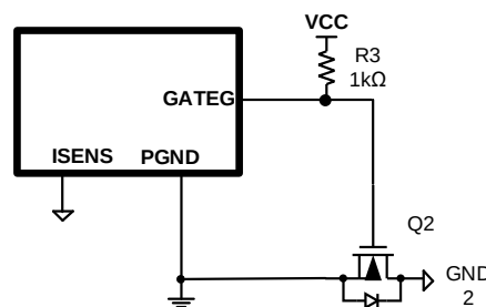
Figure 7: Battery Short-to-Ground Protection
