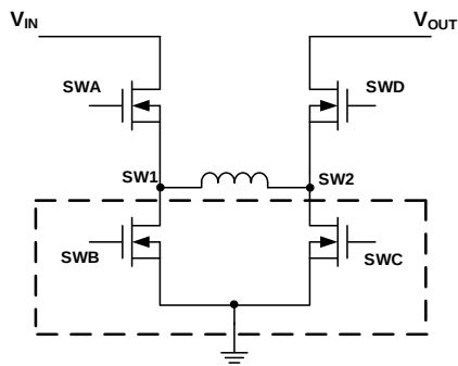
Figure 3: Buck-Boost Topology
