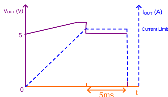
Figure 9: Over-Current Limit
