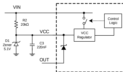
Figure 2: VCC External Connection
