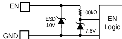
Figure 3: Zener Diode between EN and GND
