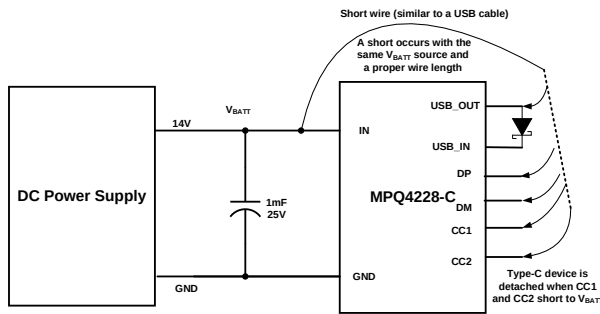
Figure 8: Short-to-Battery Set-Up
