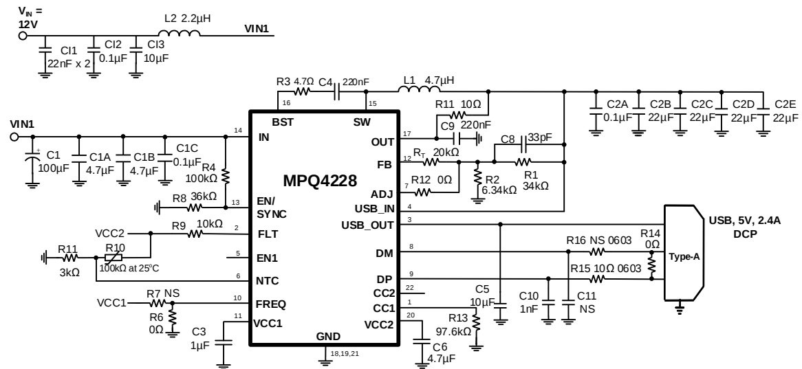
Figure 18: V_{IN} = 12V , V_{OUT} = 5V , I_{OUT} = 2.4A , f_{sw} = 420kHz (Type-A Port with BC1.2 DCP Mode, Divider 3 Mode)
