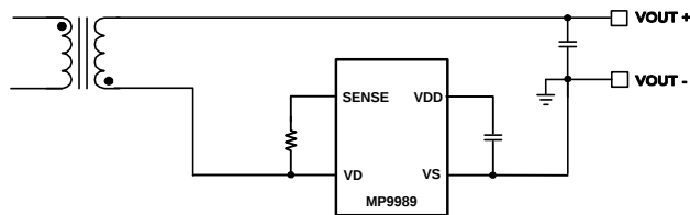
Figure 3: Low-Side Rectification
