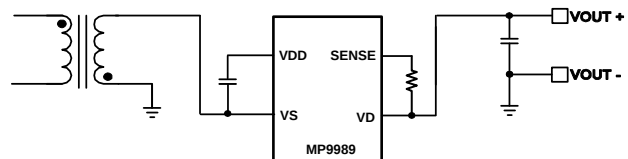
Figure 4: High-Side Rectification
