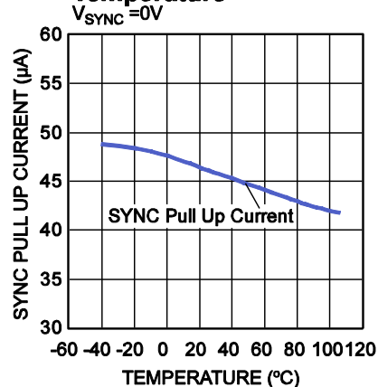
SYNC Pull Up Current vs. Temperature
