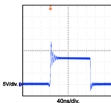
SW Output Waveform I_{OUT}=20A , R_{BST}=3.3\Omega
