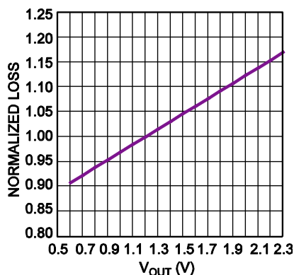
Normalized Power Loss vs. Output Voltage
