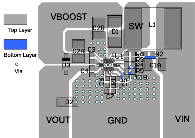
Figure 3: Layout Recommendation
