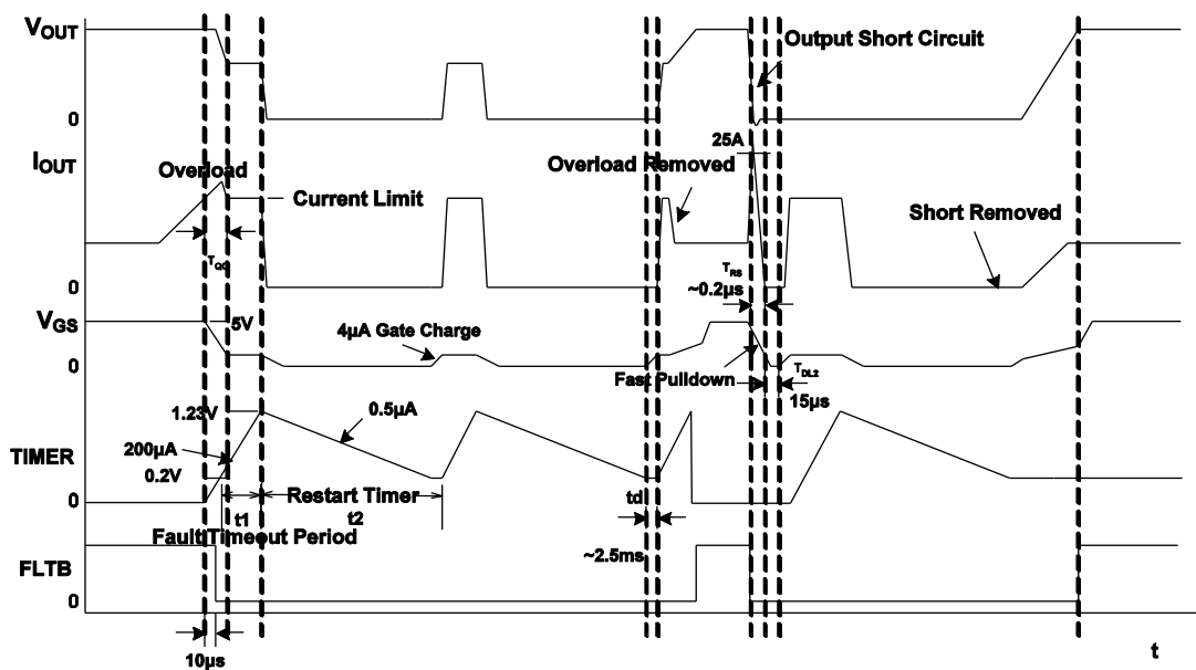
Figure 3: Over-Current Protection (Auto-Retry Mode, AUTO = High)
