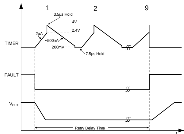
Figure 12: MP5048 Auto-Retry
