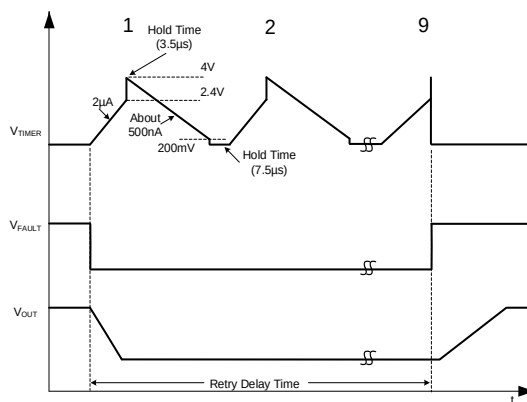
Figure 12: Auto-Retry
