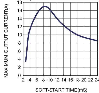
Maximum Output Current vs. Soft Start Time V IN =12V, C OUT =4700μF, En On, Single Pulse
