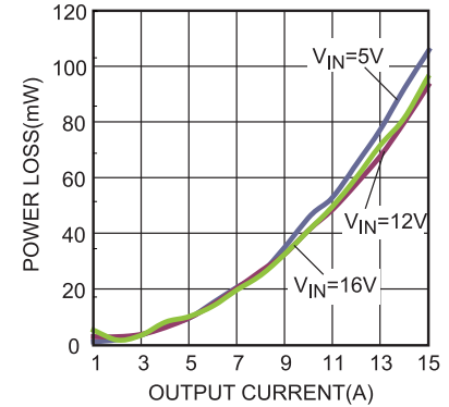
Power Loss vs. Load Current
