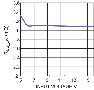
R DS_ON vs. Input Voltage I OUT =1A
