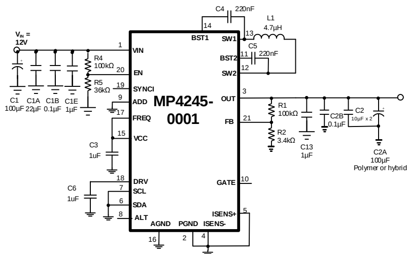
Figure 19: V_{IN} = 12V , V_{OUT} = 12V , I_{OUT} = 3A without the I 2 C (10) (11)
