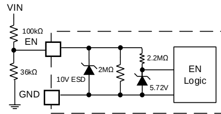
Figure 8: EN Internal Circuit
