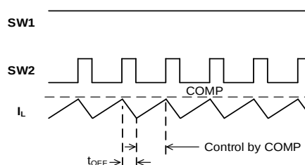
Figure 6: Boost Waveform
