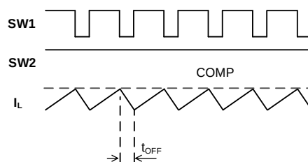
Figure 5: Buck Waveform
