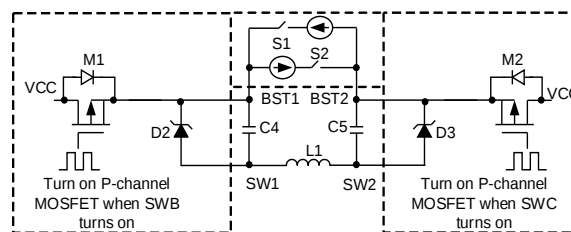
Figure 9: Internal Bootstrap Charging Circuit
