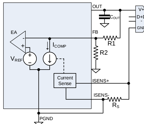
Figure 10: Sinking a Current on FB
