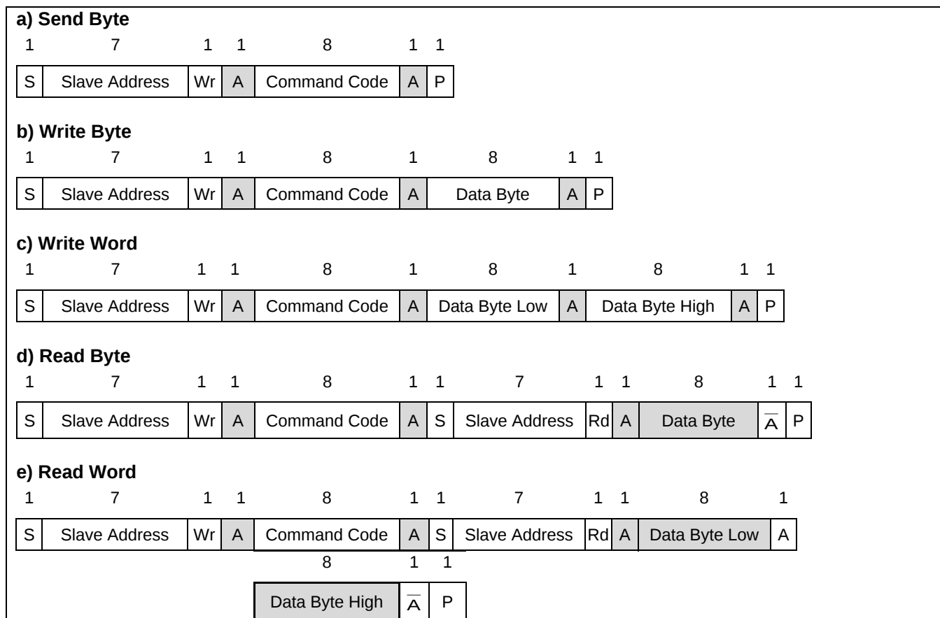
Figure 13: PMBus Message Format
