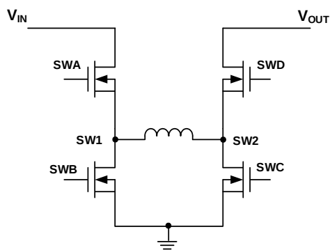
Figure 3: Buck-Boost Topology
