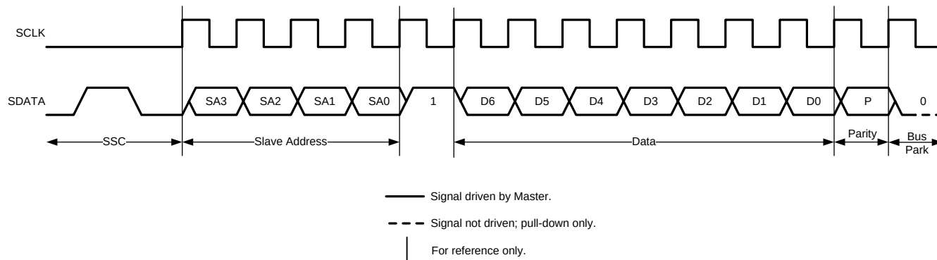
Figure 19. Register 0 Write
