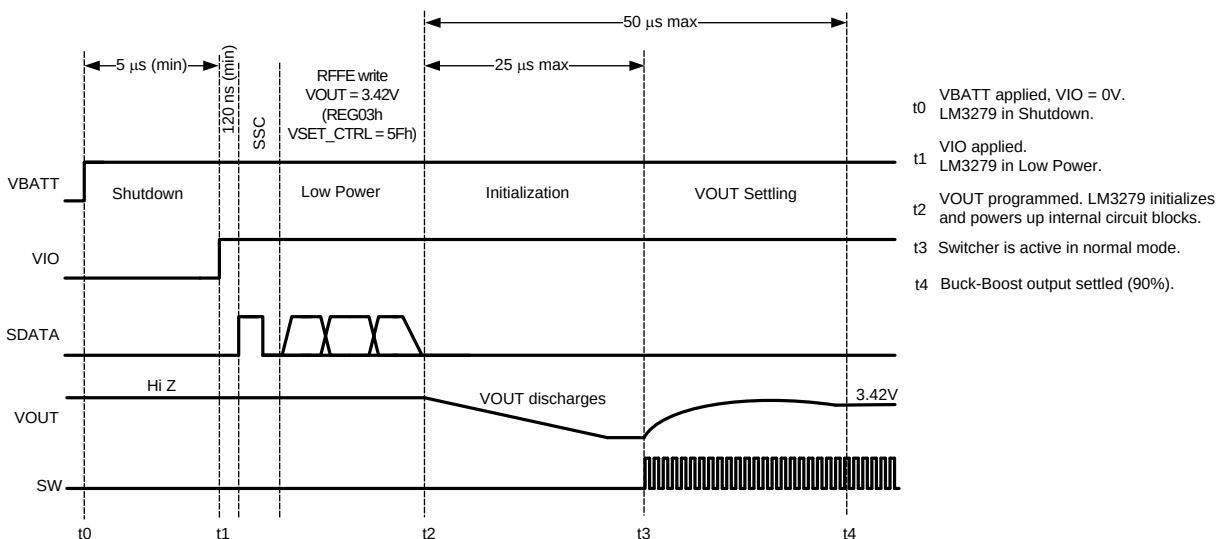
Figure 1. Cold Power-Up
