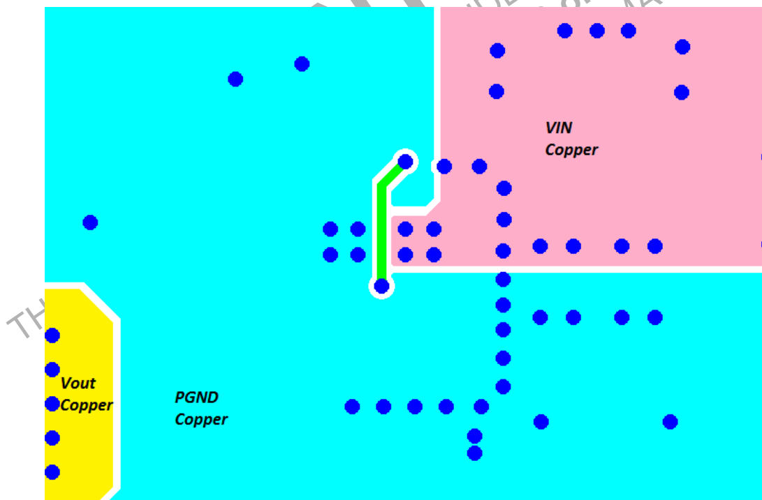
Figure 32. PCB Layout Example (Bottom View)
