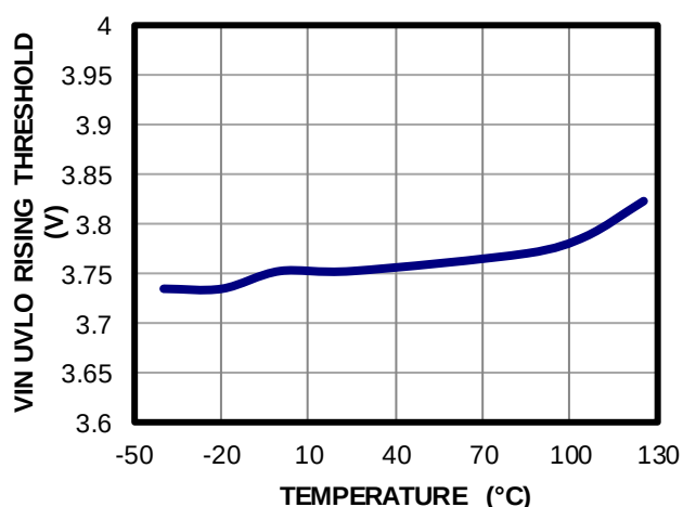
VIN UVLO Rising Threshold vs. Temperature
