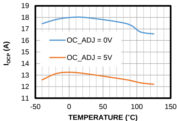
OCP Threshold vs. Temperature
