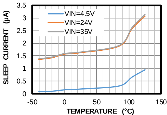
Sleep Current vs. Temperature
