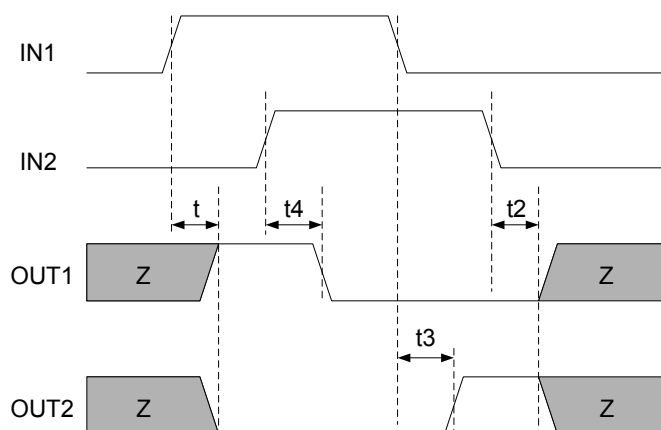
Figure 1: Input/Output Timing
