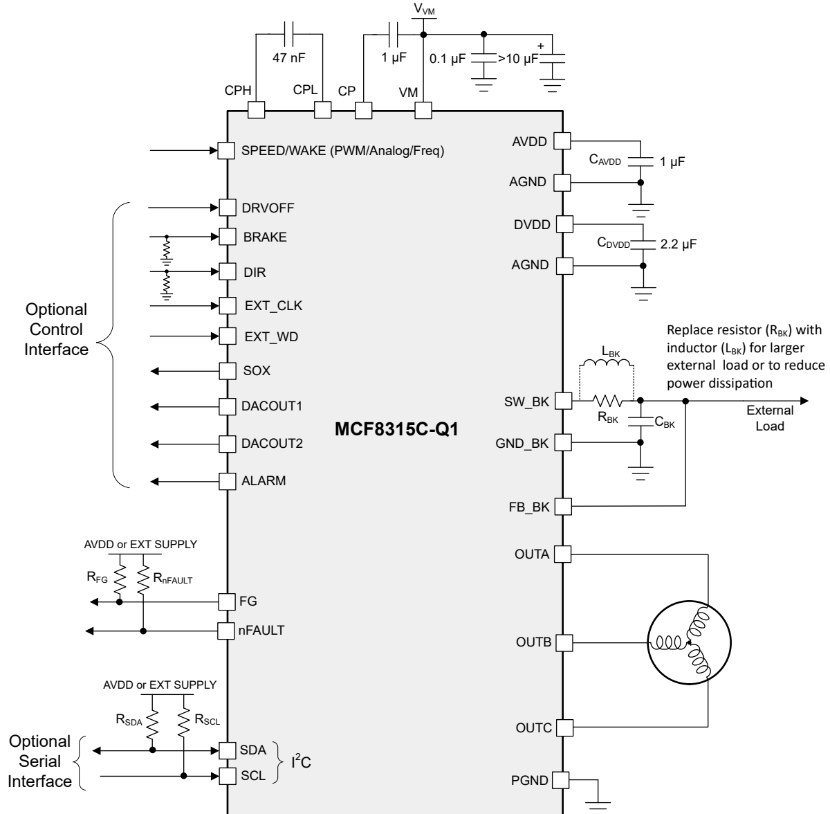
Figure 9-1. Example Application Schematic
