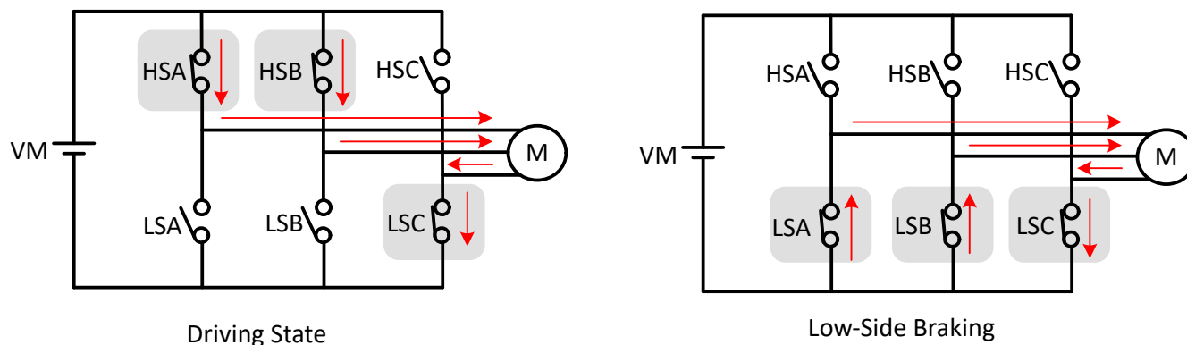
Figure 6-46. Low-Side Braking
