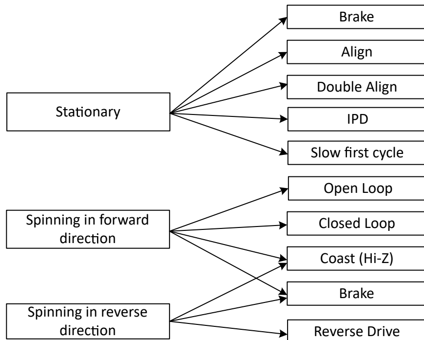
Figure 6-23. Starting the motor under different initial conditions
