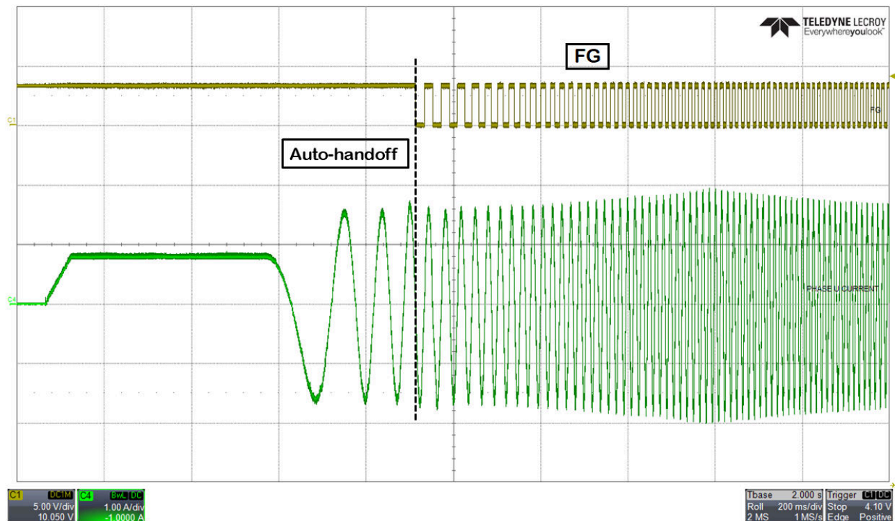
Figure 9-7. Auto-handoff
