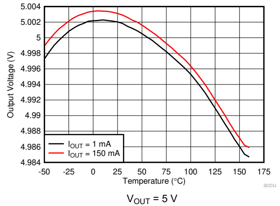
Figure 5-8. Output Voltage vs Ambient Temperature
