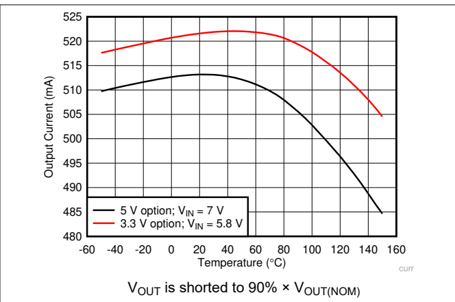
Figure 5-14. Output Current Limit vs Ambient Temperature
