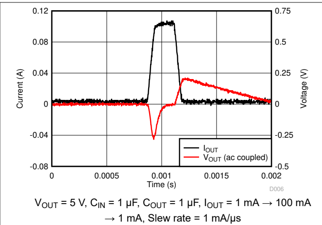
Figure 5-20. Load Transient
