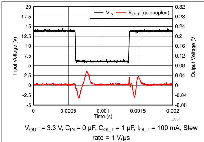
Figure 5-19. Line Transient
