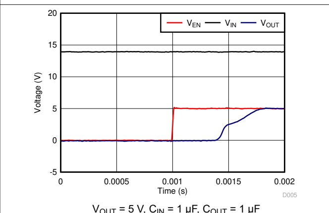
Figure 5-18. Startup With Enable
