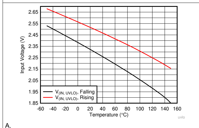
Figure 5-17. UVLO vs Ambient Temperature
