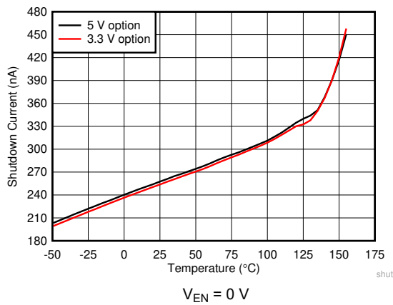
Figure 5-1. Shutdown Current vs Ambient Temperature
