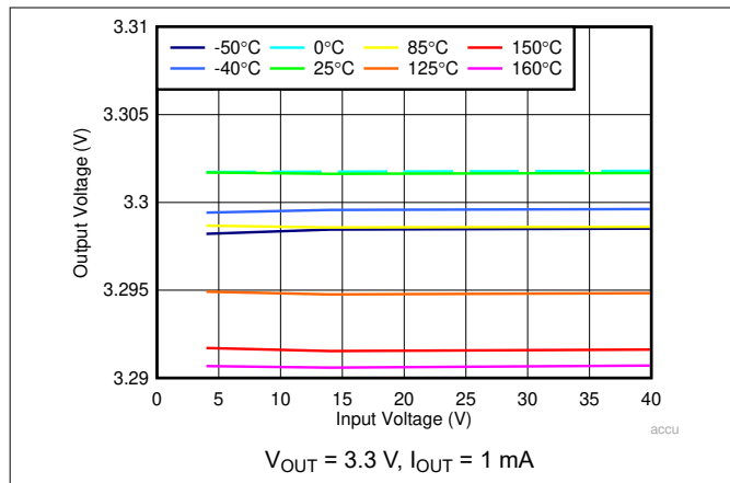
Figure 5-13. Output Voltage vs Input Voltage
