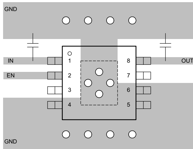
Figure 7-9. TPSB81-Q1 Example Layout Diagram
