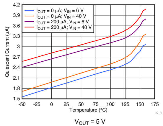
Figure 5-2. Quiescent Current vs Ambient Temperature
