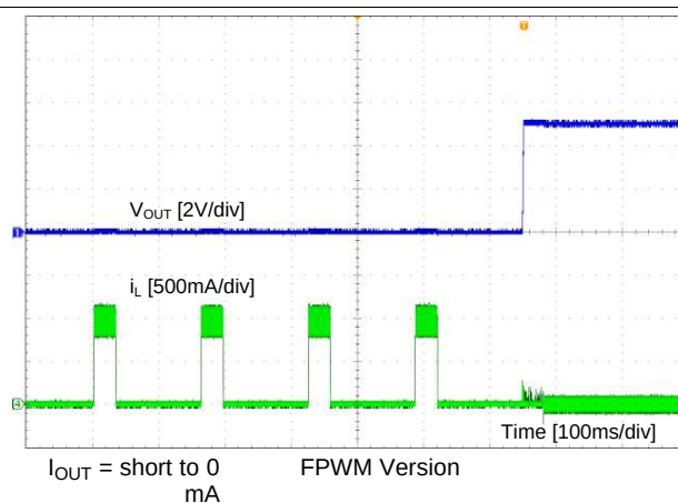
Figure 26. Short Recovery
